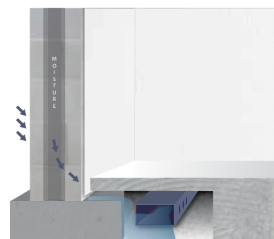
AFTER (OPTION 2) FULL HEIGHT PROTECTION
